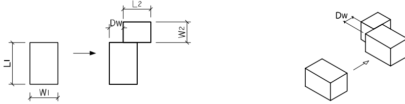
Figure 4. Parametric rule schema R1AB
