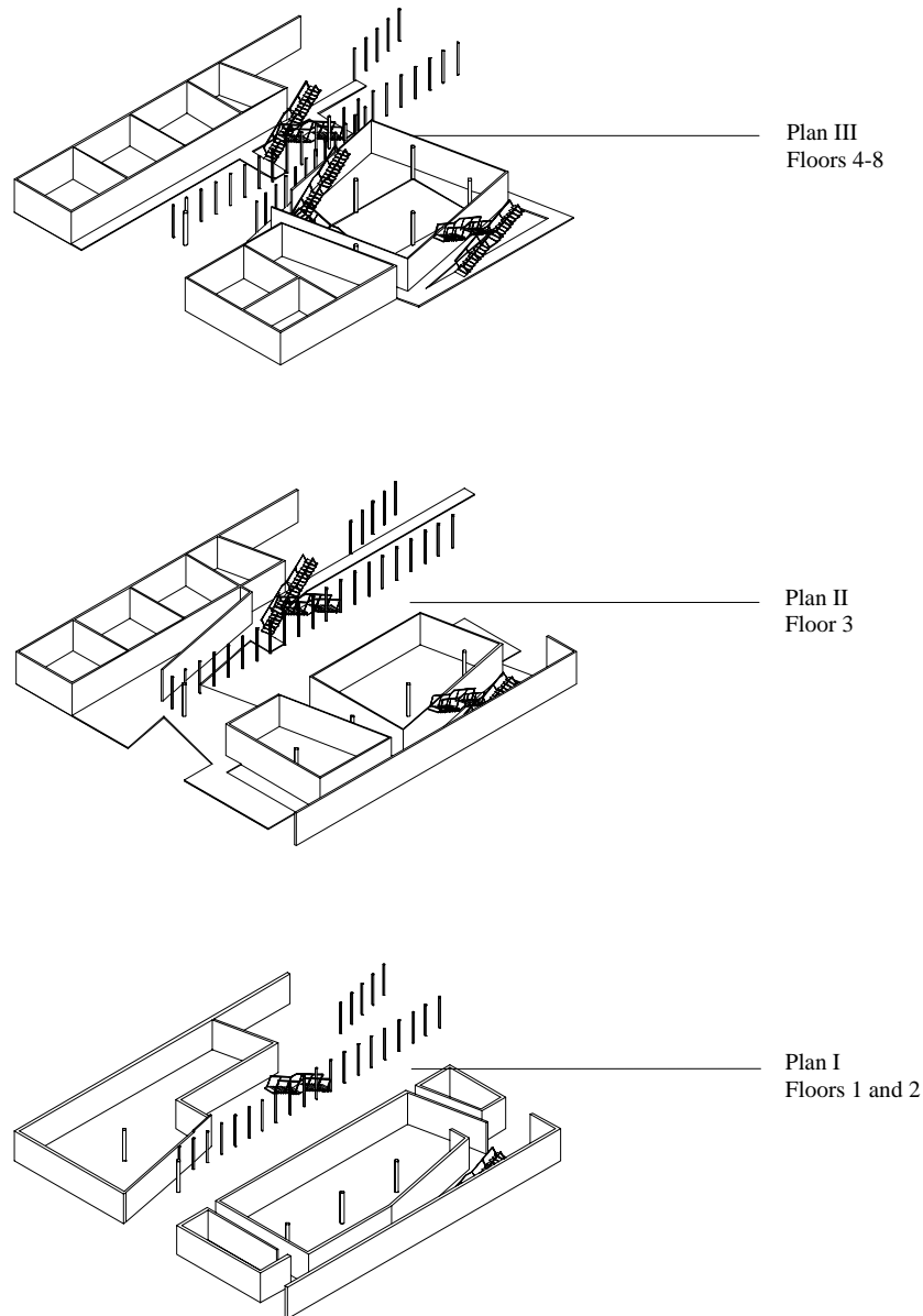
Figure 19. The output descriptions of the plans I, II, III in axonometric
