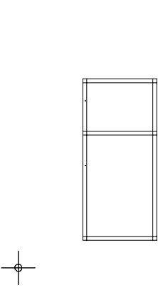
B: \langle U_{12} \rangle
