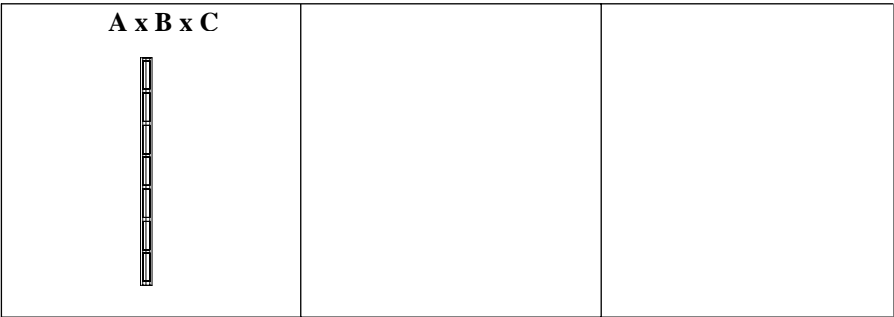
U_{12} \times U_{12} \times U_{12}
