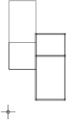
A x B: \langle U_{12} \times U_{12} \rangle
